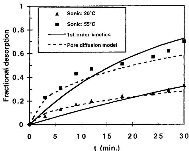
Figure 10. Fractional desorption of phenol from Dowex Optipore resin vs. time: comparison of first-order surface-kinetic model and pore-diffusion model with experimental data at 20°C and 55°C with 50% (60 W) of the peak power, corresponding to Figure 7.
